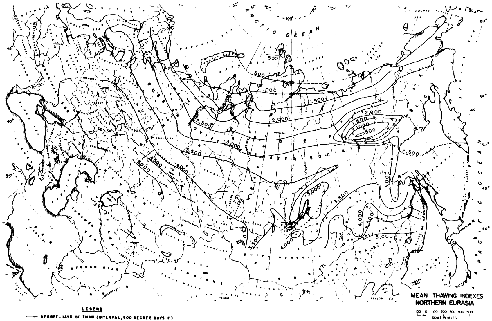
Figure A-2b. Distribution of mean air thawing indexes (°F) - Northern Eurasia.
