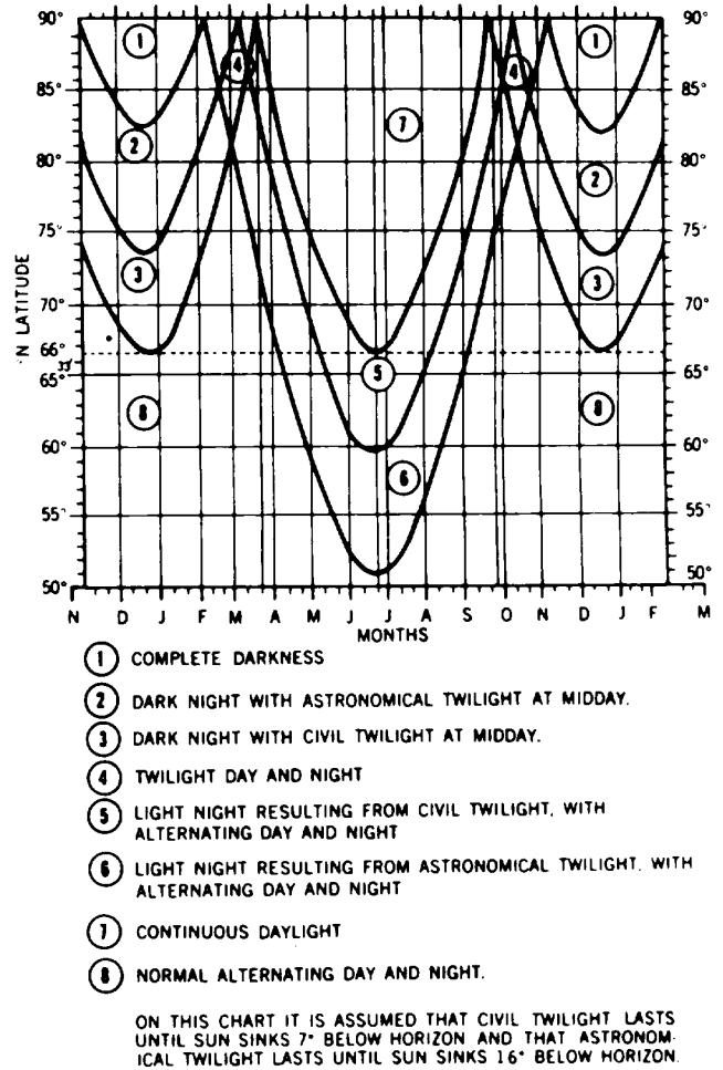
Figure 2-11. Solar illumination in the Arctic.
