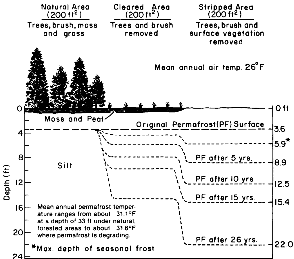
Figure 5-1. Permafrost degradation under different surface treatments over a 26-year period at Fairbanks, Alaska.
