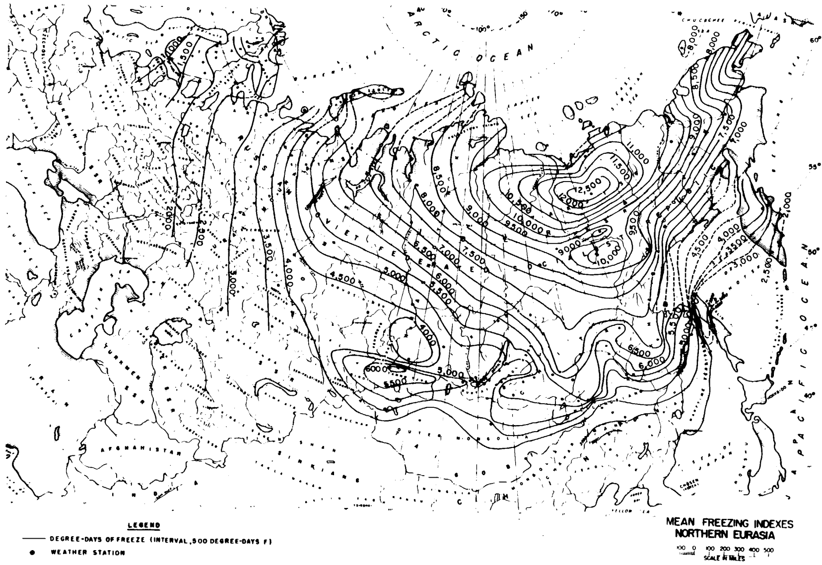
Figure A-1b. Distribution of mean air freezing indexes ( ^{\circ} F) - Northern Eurasia.
