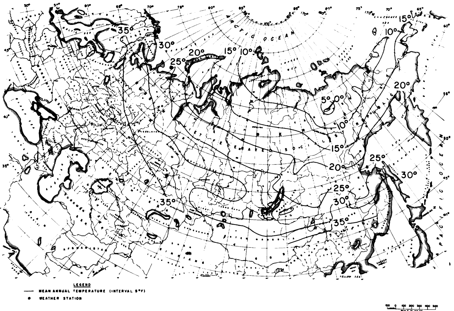
Figure 2-4. Distribution of mean annual air temperature (° F) in northern Eurasia.
